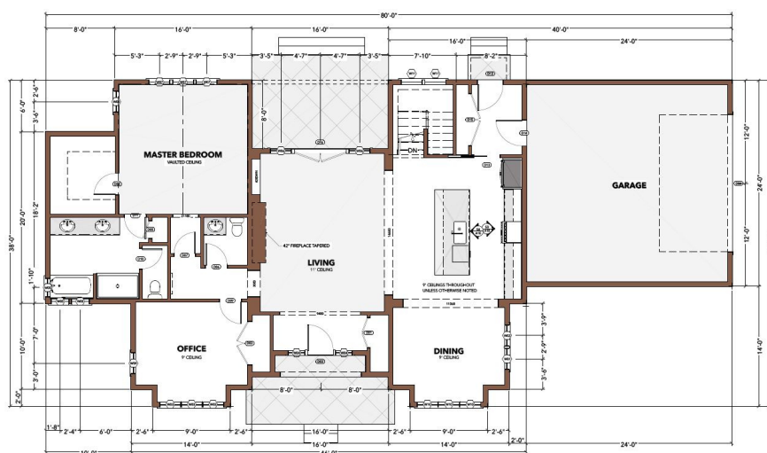
MAIN FLOOR
